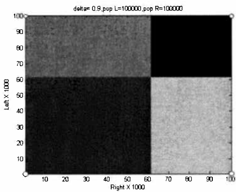
(b) Basins of attraction when \delta = 0.9 .
