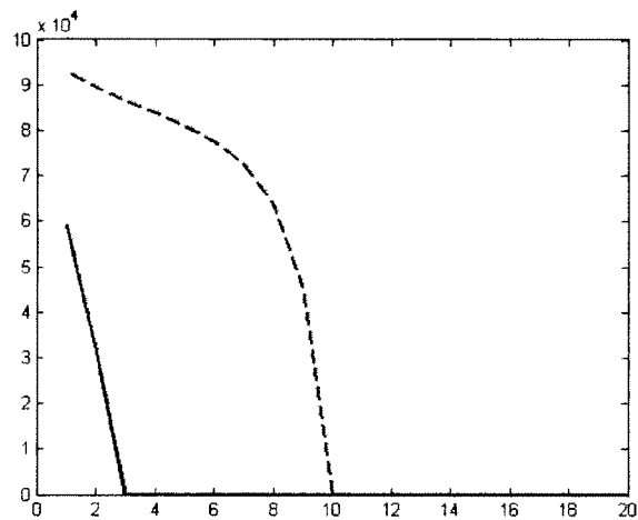
(b) Trajectories when \delta = 0.5 . The system converges to the no vote equilibrium.
