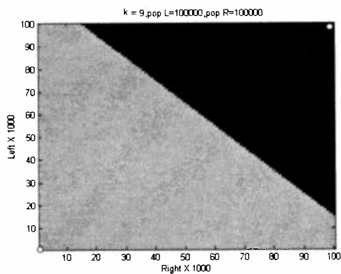
(b) Basins of attraction when k = 9 .
