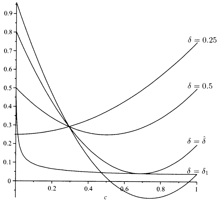
Figure 1: Equilibria as a function of \delta , with n = 1,000 . Interior equilibria are obtained as the intersection between two curves, the marginal benefit of voting, which decreases exponentially with c , and the marginal cost of voting, which changes with respect to \delta , but passes through (c_m, c_m) for all values of \delta . Corner equilibria are achieved by comparing marginal costs and benefits at the extremes, c = 0 and c = 1 .
