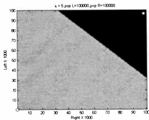
(a) Basins of attraction when k = 5 .
