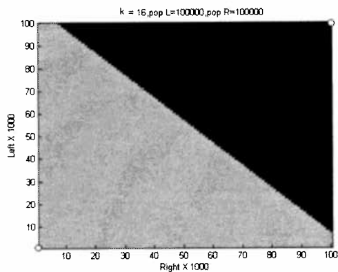
(c) Basins of attraction when k = 16 .
