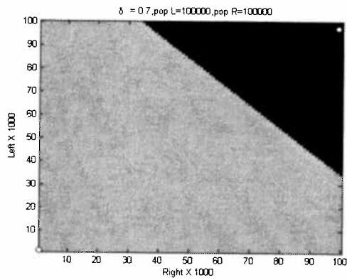
(a) Basins of attraction when \delta = 0.7 .
