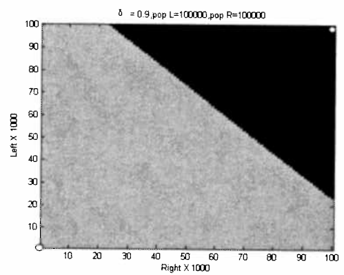
(b) Basins of attraction when \delta = 0.9 .
