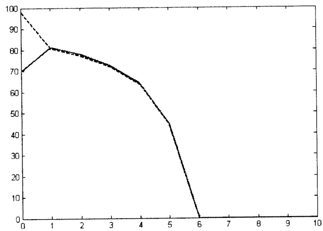
(b) Trajectories when \delta = 0.5 . The system converges to the no vote equilibrium.
